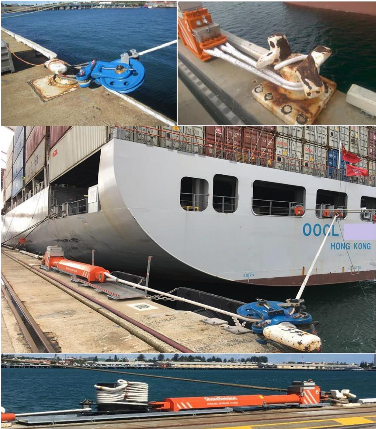
Fig 1: Various components of the ShoreTension® system
