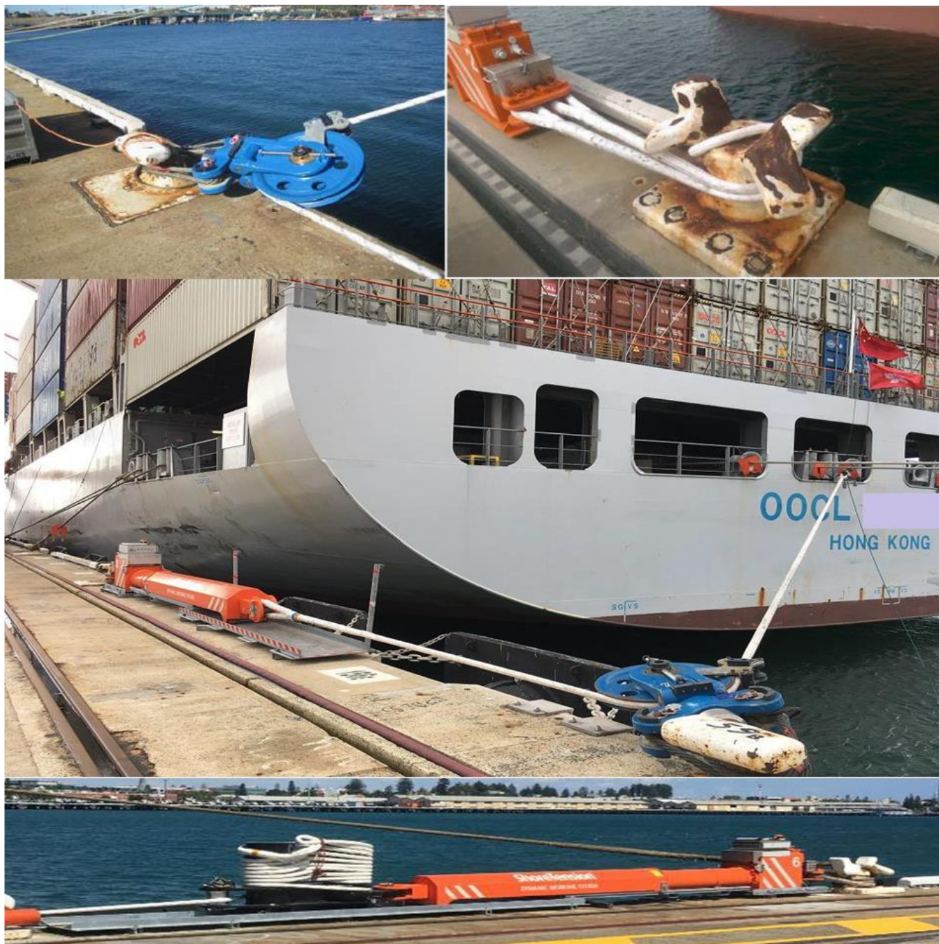
Fig.1: Various components of the ShoreTension® system
